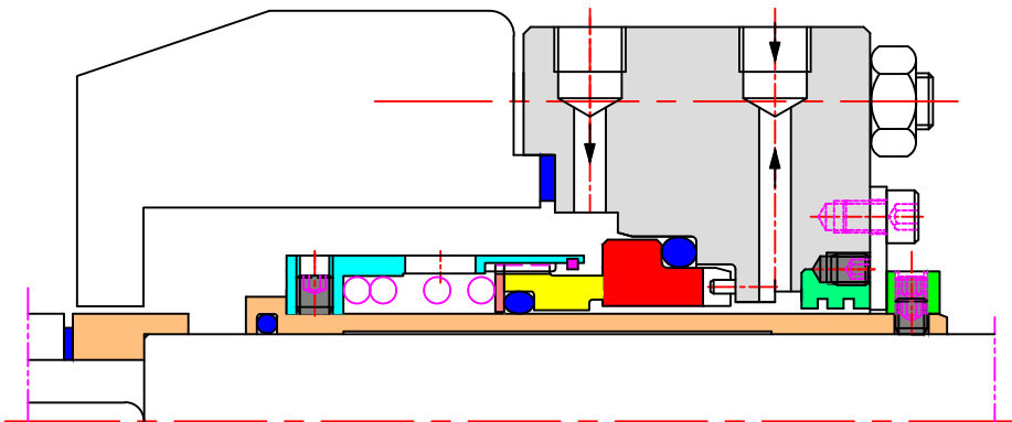
80 SERIES SINGLE SPRING MECHANICAL SEAL TYPE 8101 CARTRIDGE ARRANGEMENT WITH DIFFERENT API PLAN 11& 62
